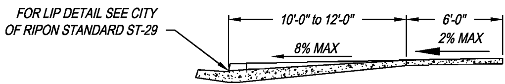
SECTION VIEW
